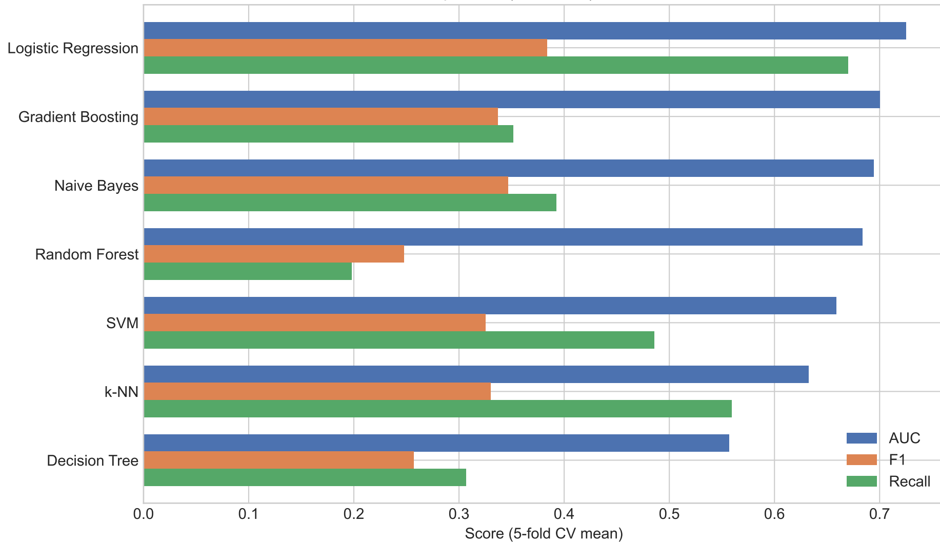
Model comparison (5-fold CV): AUC, F1, Recall
